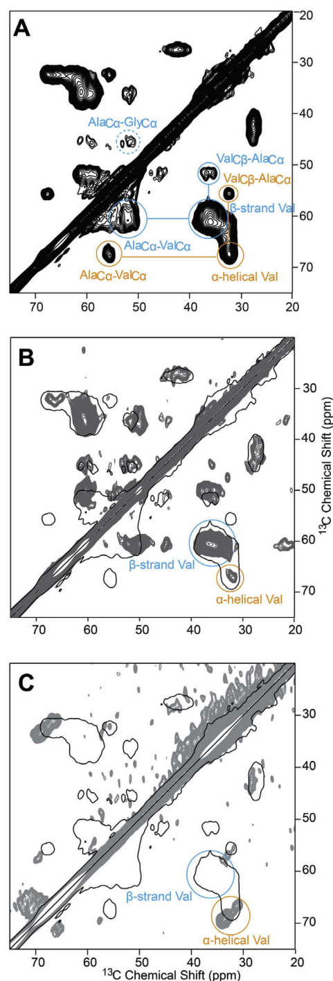
Fig. 4. 2D ^{13}\text{C}/^{13}\text{C} -correlation spectra (acquired with proton-driven spin-diffusion with a mixing time of 1 s, at a field strength of 14.1 T, with a spinning frequency of 9 kHz) of sparsely ^{13}\text{C} labeled \alpha -synuclein in frozen solution in different environment. A) For disordered monomeric \alpha -synuclein in a glycerol-water solution the Valine C \alpha /C \beta cross-correlation signal is largely inhomogeneously broadened, shift regions typical for \alpha -helical as well as for \beta -strand like conformations are covered. Further, interresidual cross-correlation signals to neighboring Alanine residues are indicative of a correlation between similar conformations for neighboring residues. B) For a frozen suspension of fibrillar \alpha -synuclein (grey spectrum) the \beta -sheet content is increased with respect to monomeric \alpha -synuclein (black outline), whereas for \alpha -synuclein in contact with lipid bilayers (C) only \alpha -helical shifts are observed. Adapted with permission from Ref. [104], copyright (2018) Elsevier.
